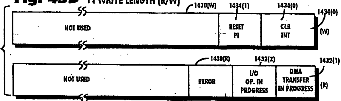
Fig. 45E PI CONTROL/STATUS REGISTER (R/W)
